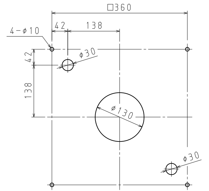
推奨据付寸法 (1:6) RECOMMENDED INSTALLATION DIMENSIONS (1:6)
